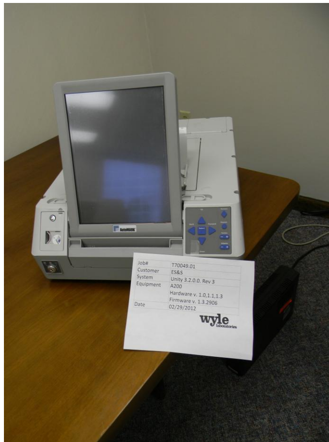
Photograph No. 4: AutoMARK A200 VAT
